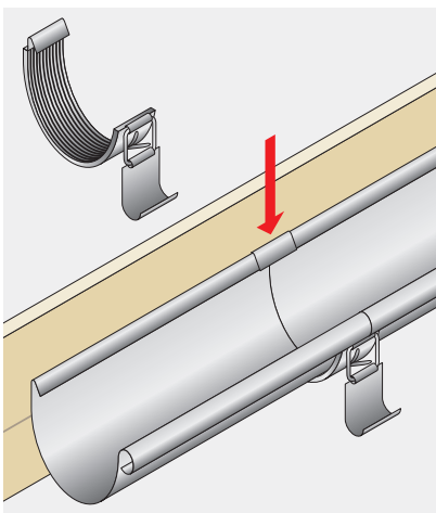
4. An EDPM rubber sealed union connector is used to connect the gutter lengths and angles together. Locate the union connector over the rear edge of the gutter.
