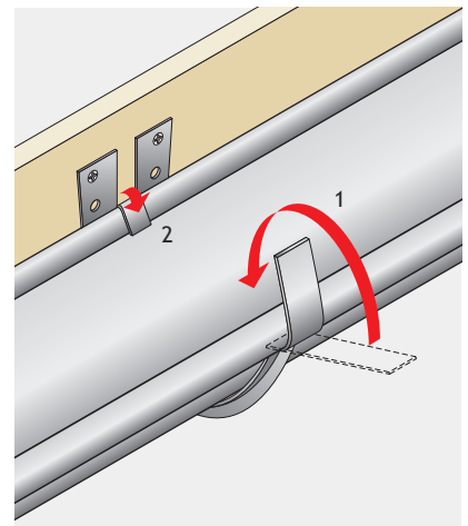
6. Locate the gutter into the fascia bracket and seat level, then fold the front tab of the fascia bracket around the front roll and into the gutter. Fold the rear tab of the fascia bracket down and over the rear edge of the gutter.
