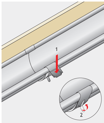
5. Locate the clasp over the front roll edge of the gutter. Push down on top of the clasp and squeeze the clasp shut. Fold the locking tab over to fully secure.
